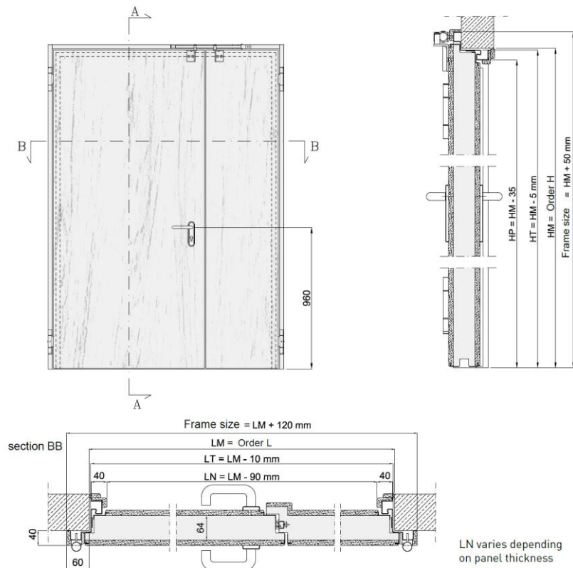
Fire-proof steel door, double leaves, REI120, with panel
